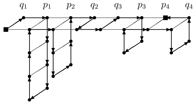
Figure 1: Path in pair of combs for n = 8 and k = 5 .
