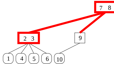
Figure 3.10. \mathcal{T}_{2,4}(10)
