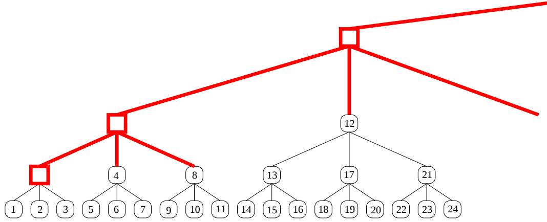
Figure 3.4. \mathcal{F}_{0,3}
