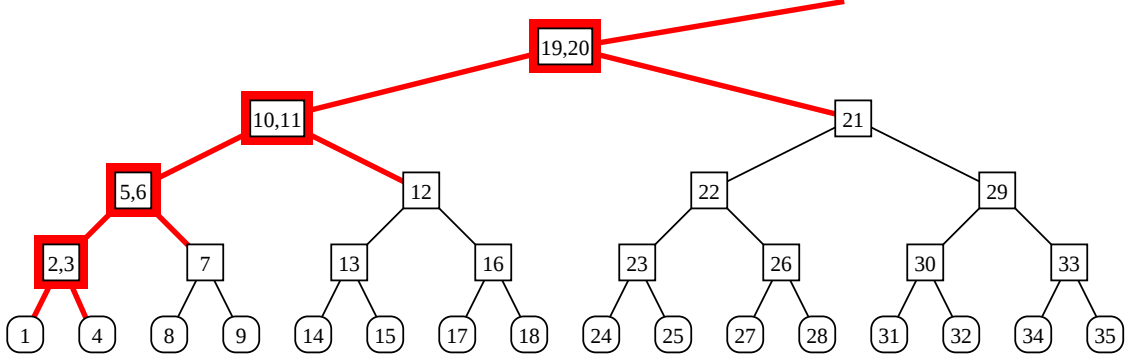
Figure 3.3. \mathcal{F}_{2,2}
