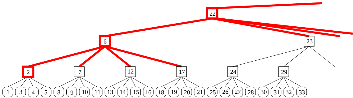
Figure 3.8. \mathcal{F}_{1,4}
