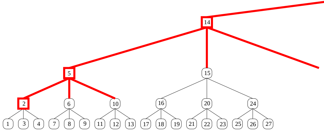
Figure 3.4. \mathcal{F}_{0,3}
