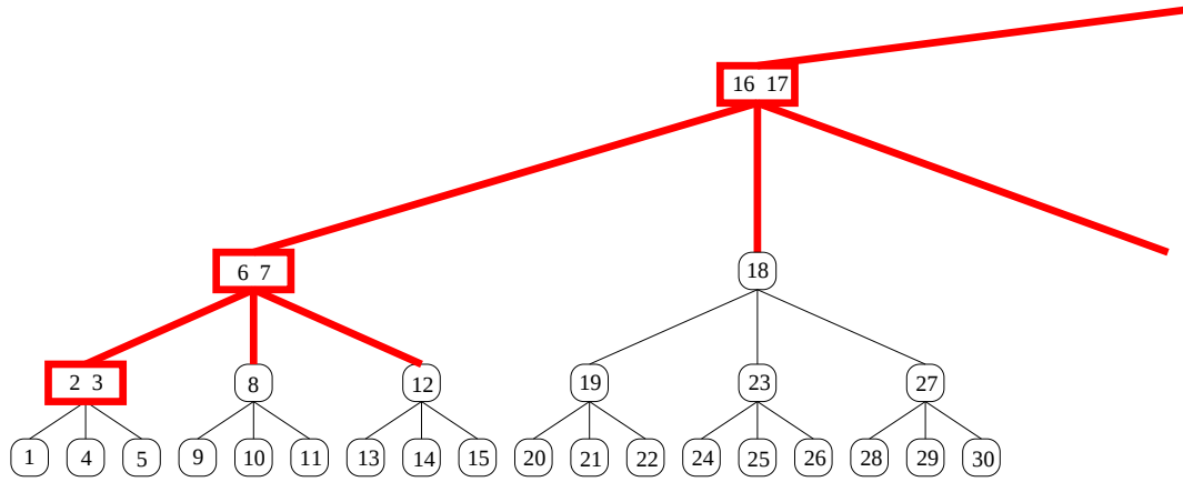
Figure 3.6. \mathcal{F}_{2,3}
