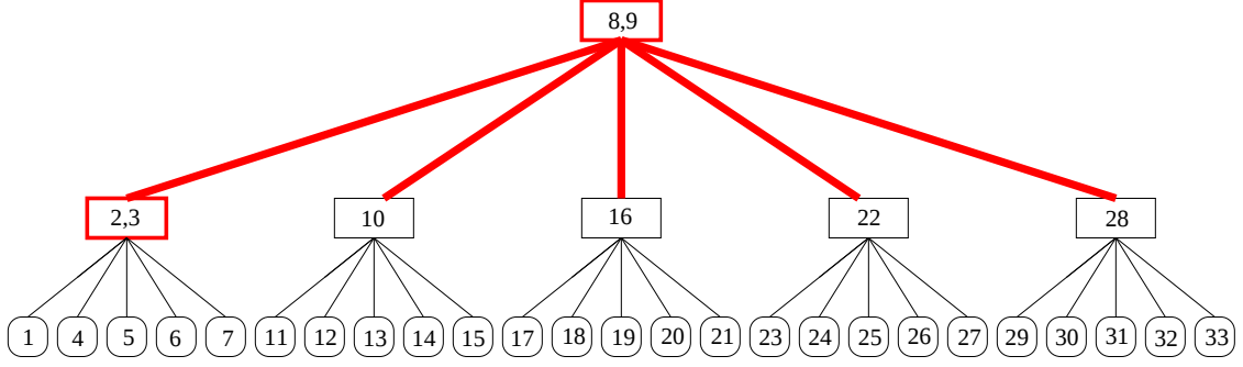
Figure 3.9. \mathcal{T}_{2,5}(33)
