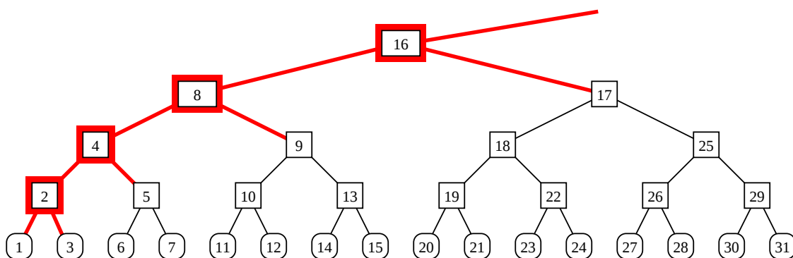
Figure 3.1. \mathcal{F}_{0,2}
