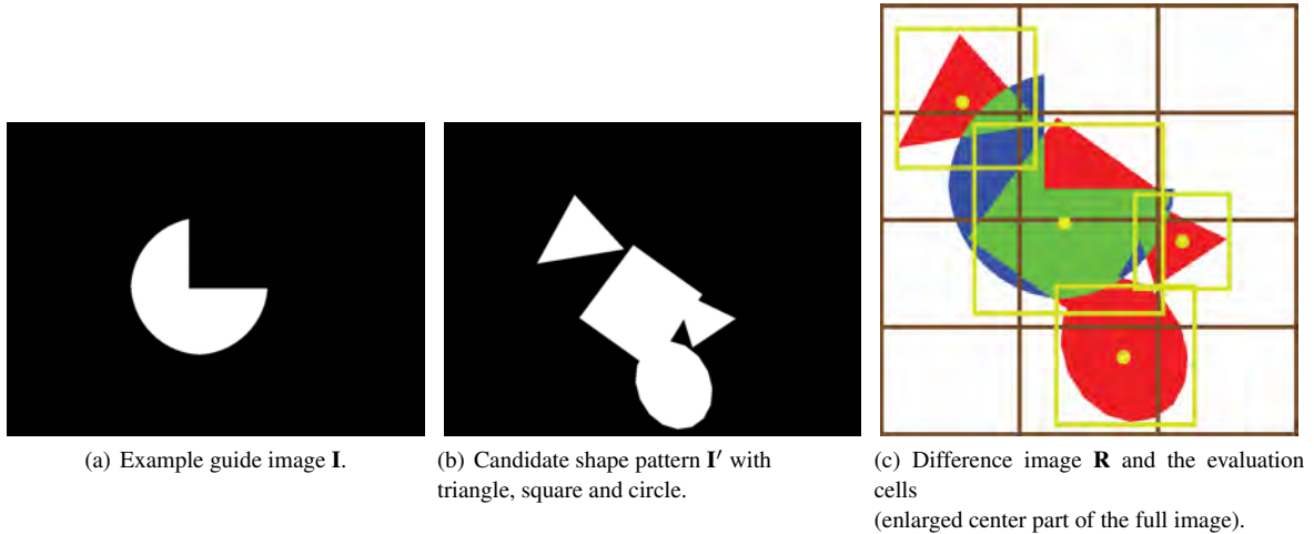
Figure 4: Optimization Heuristics. Blue in the difference images denotes pixels covered only by the guide image but not the candidate shape pattern, while red stands for pixels covered only by the candidate shape pattern but not the guide image. The dark brown squares represent the evaluation lattice. The yellow squares represent instance cells, which have their centers aligned with the geometrical centers of the shape instances.
