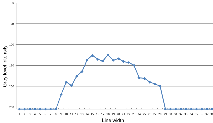
Fig. 6. The approximately bell-shaped curve showing intensity values of cross sections of a lines drawn with a 6B pencil.
