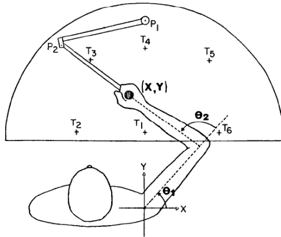
Fig. 3. Apparatus used by Flash and Hogan [1985] to measure arm trajectories in a horizontal plane. Movement of the hand was measured using potentiometers P1 and P2.
