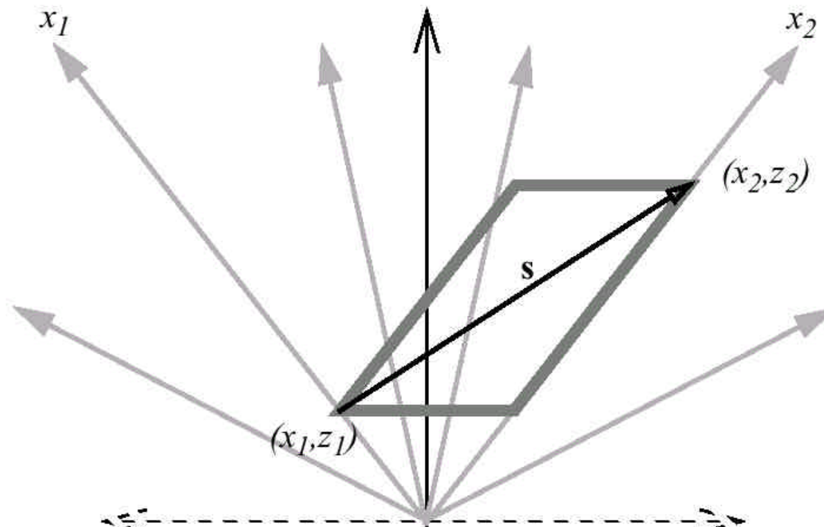
Figure 7. Solution to the simple joint pan-zoom problem. The trajectory \mathbf{s} monotonically approaches point 2 in both pan and zoom.
